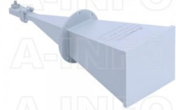
LB-42-25-C2-SFSPO Standard Gain Horn Antenna 18-26.5GHz 25dB Gain SMA Female
